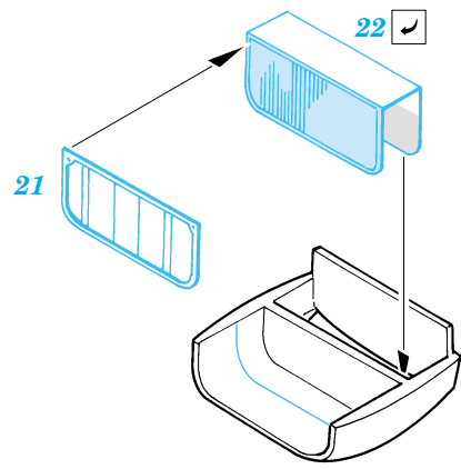
Kit part 15
